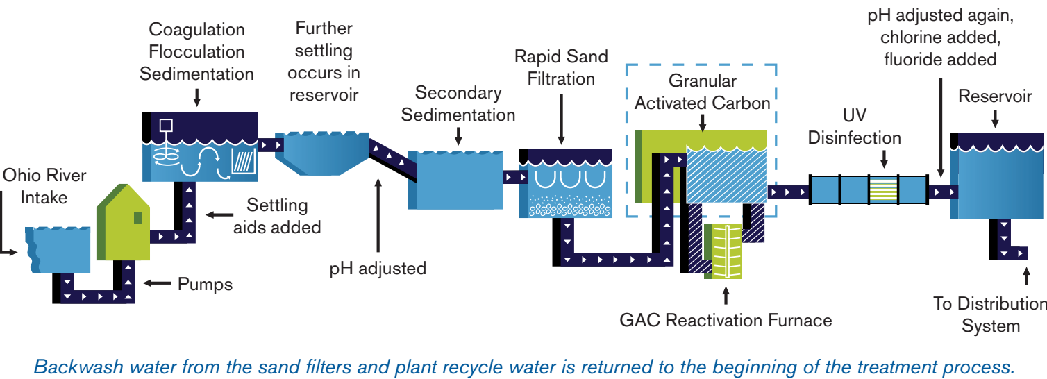
Treatment Process at the Richard Miller Plant on the Ohio River
