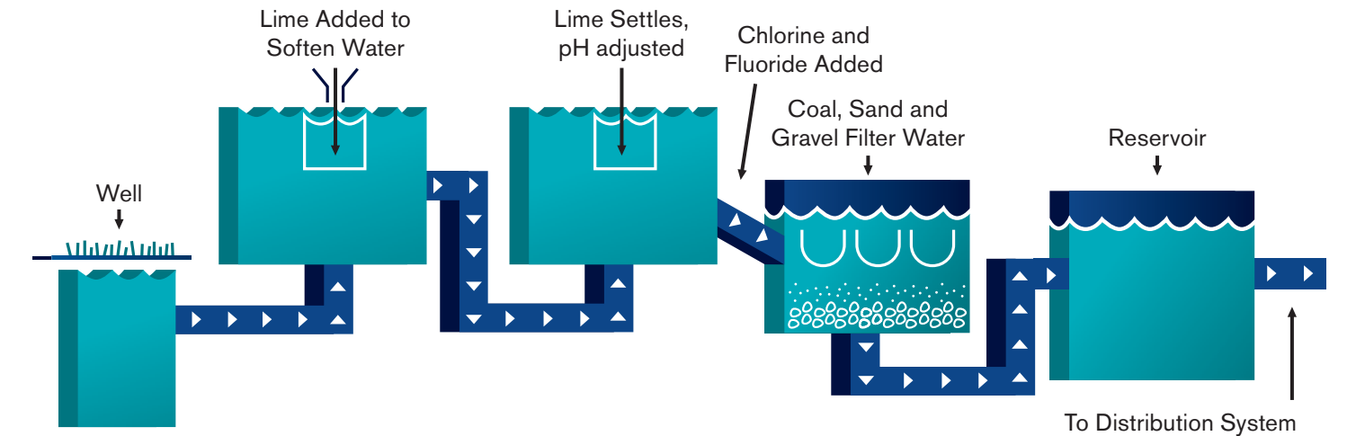
Treatment Process at the Charles M. Bolton Plant on the Great Miami Buried Valley Aquifer
